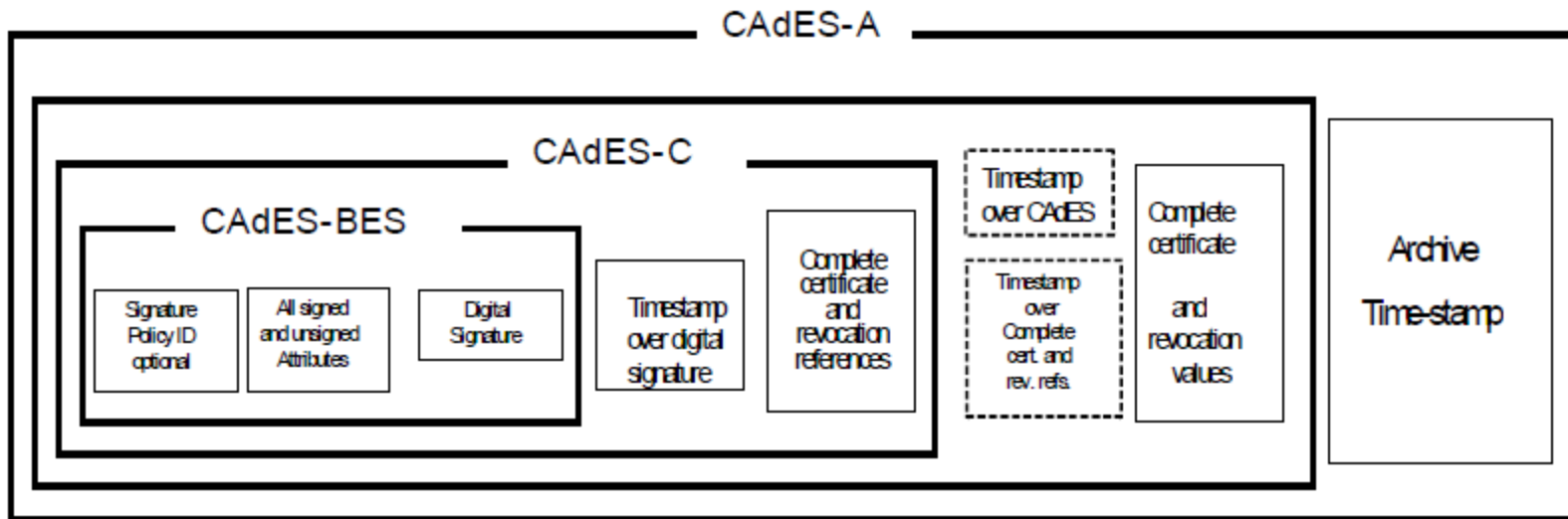
Figure 10: Illustration of CAdES-A
